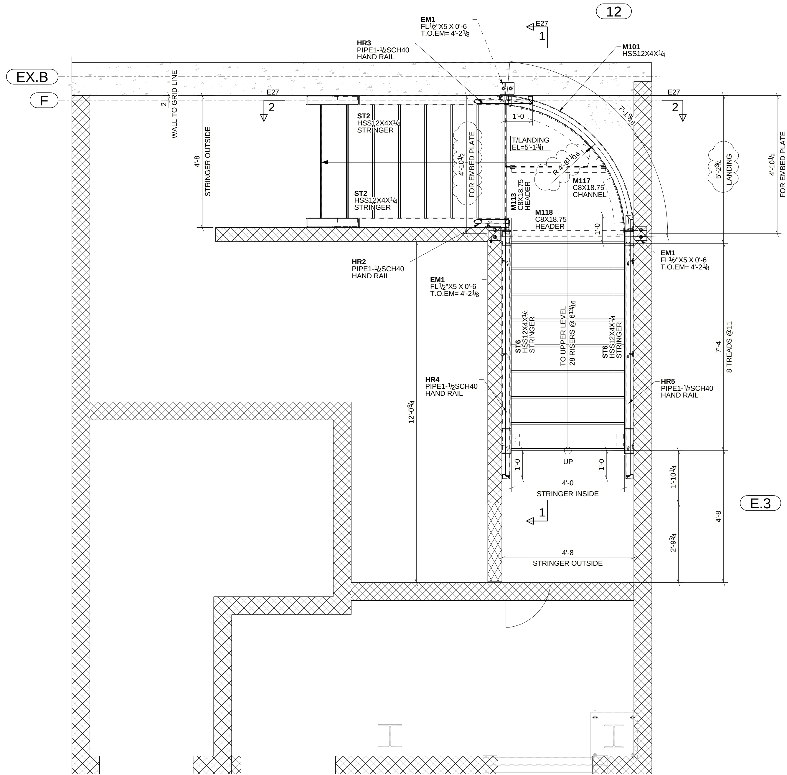
STAIR-2 LOWER LEVEL FRAMING PLAN (Ref : 2/A7.2)
