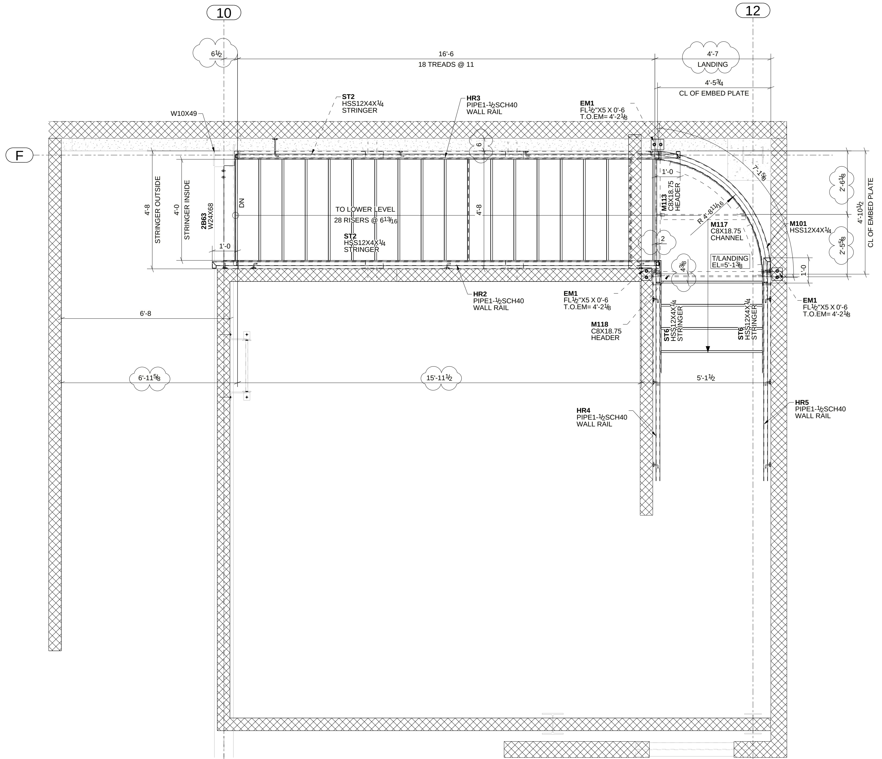
STAIR-2 UPPER LEVEL FRAMING PLAN (Ref : 3/A7.2)
